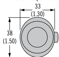
Oval Perpendicular
